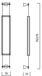
Parete - Wall
