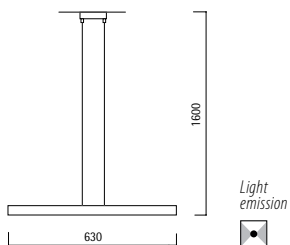
Lampada sospensione - Pendant lamp 000116 Bianco opaco - Matt white LED 4x6W 3.000°K CE V IP30
